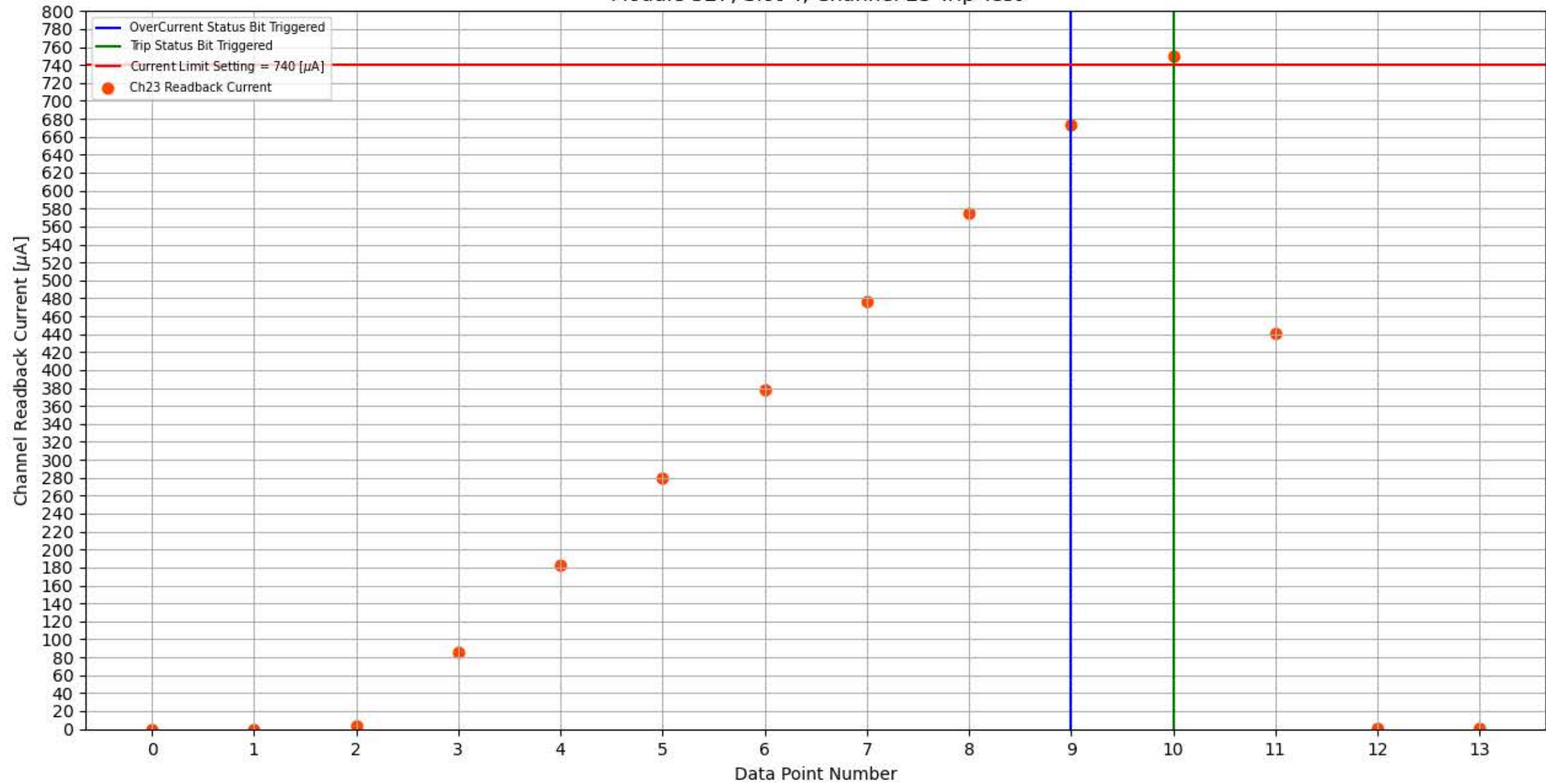
Module 327, Slot 4, Channel 23 Trip Test
