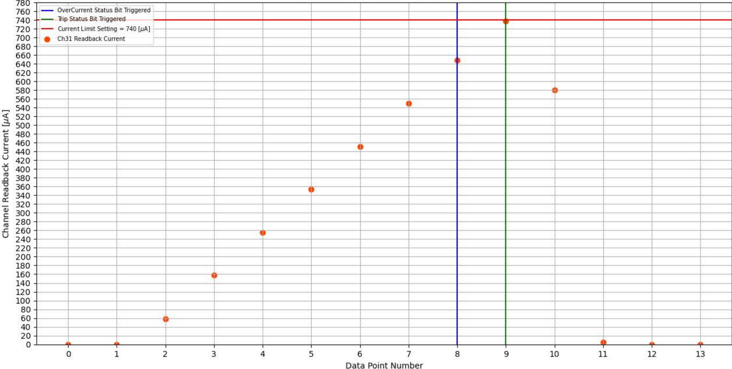
Module 327, Slot 4, Channel 31 Trip Test
