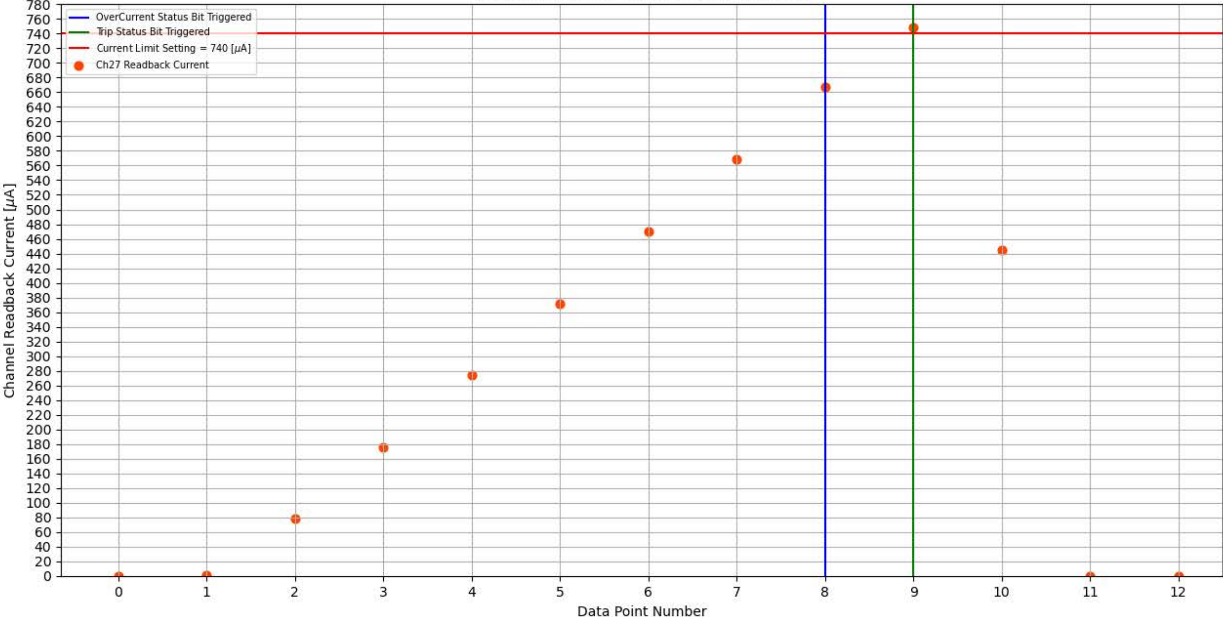
Module 327, Slot 4, Channel 27 Trip Test
