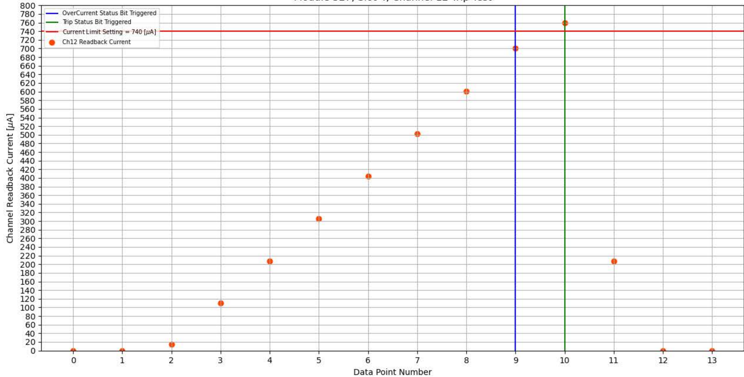
Module 327, Slot 4, Channel 12 Trip Test
