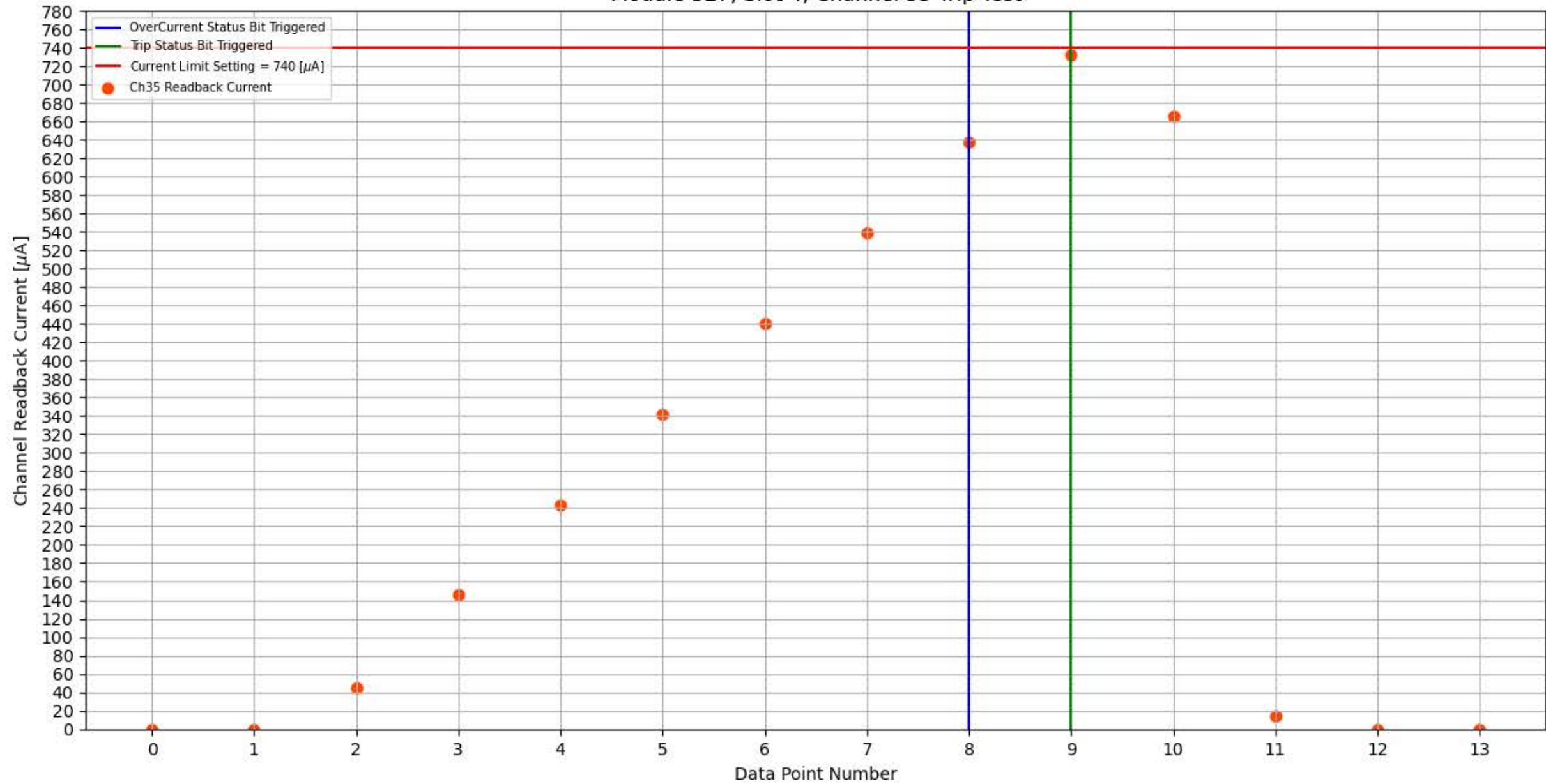
Module 327, Slot 4, Channel 35 Trip Test
