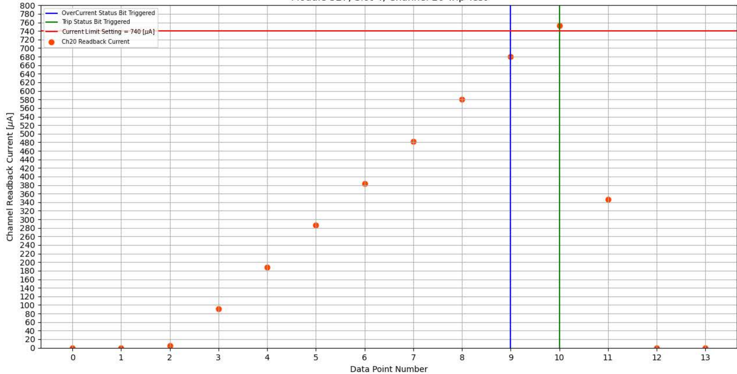
Module 327, Slot 4, Channel 20 Trip Test
