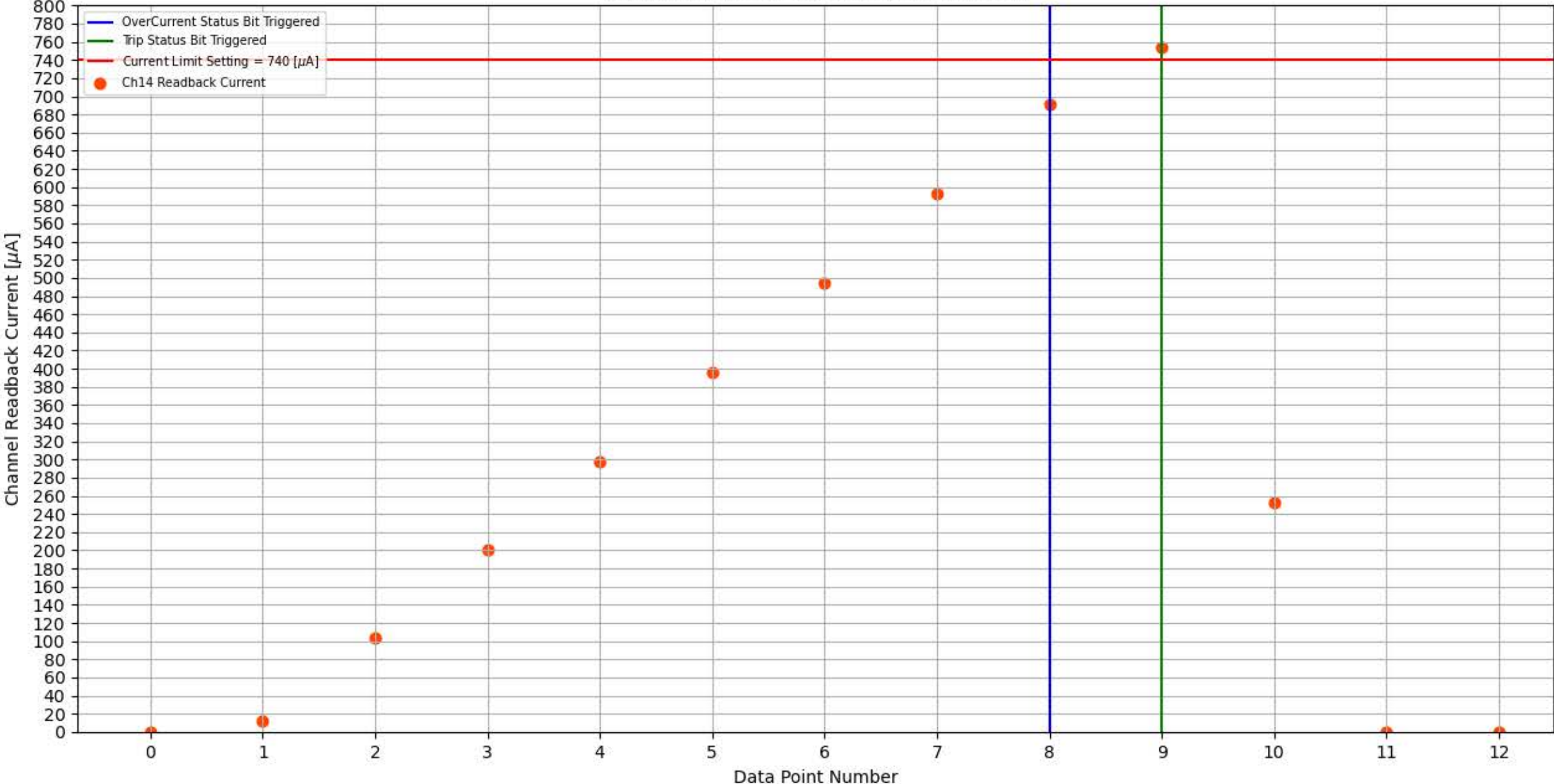
Module 327, Slot 4, Channel 14 Trip Test
