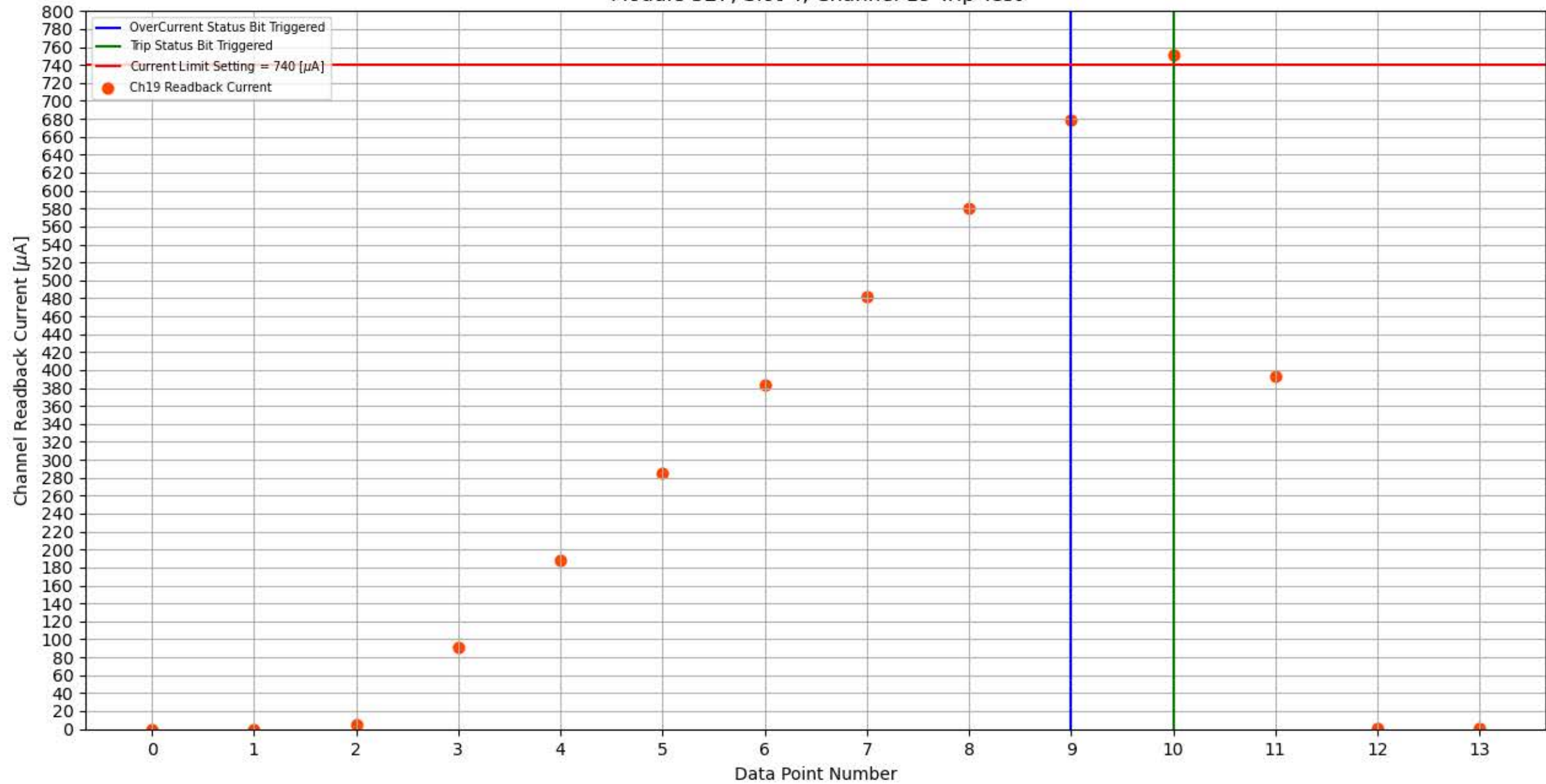
Module 327, Slot 4, Channel 19 Trip Test
