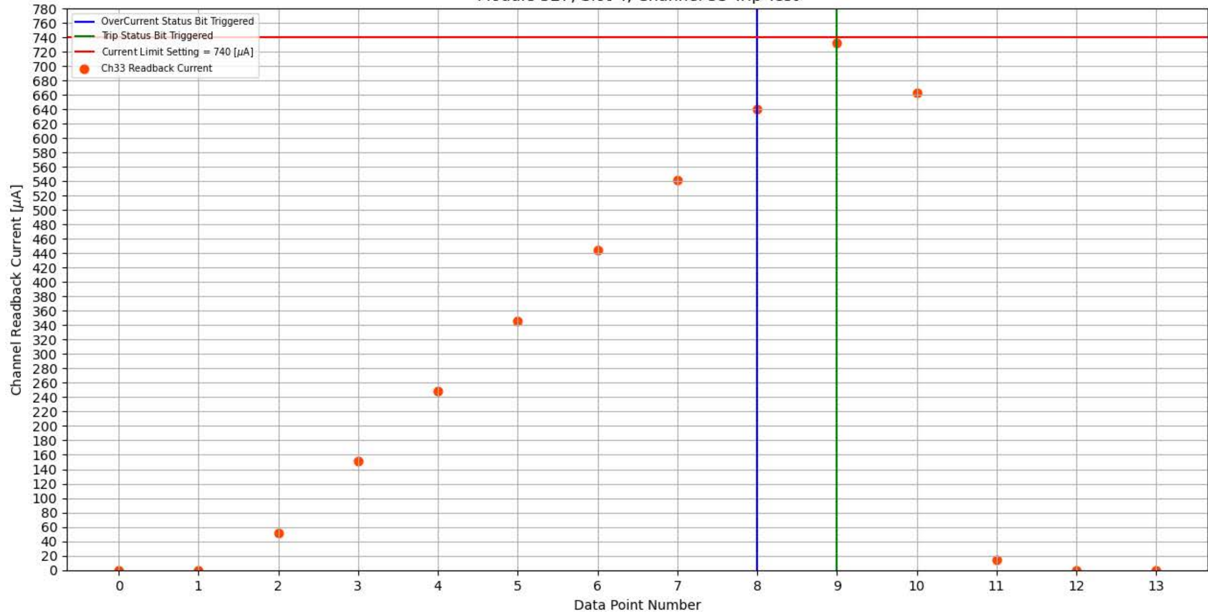
Module 327, Slot 4, Channel 33 Trip Test
