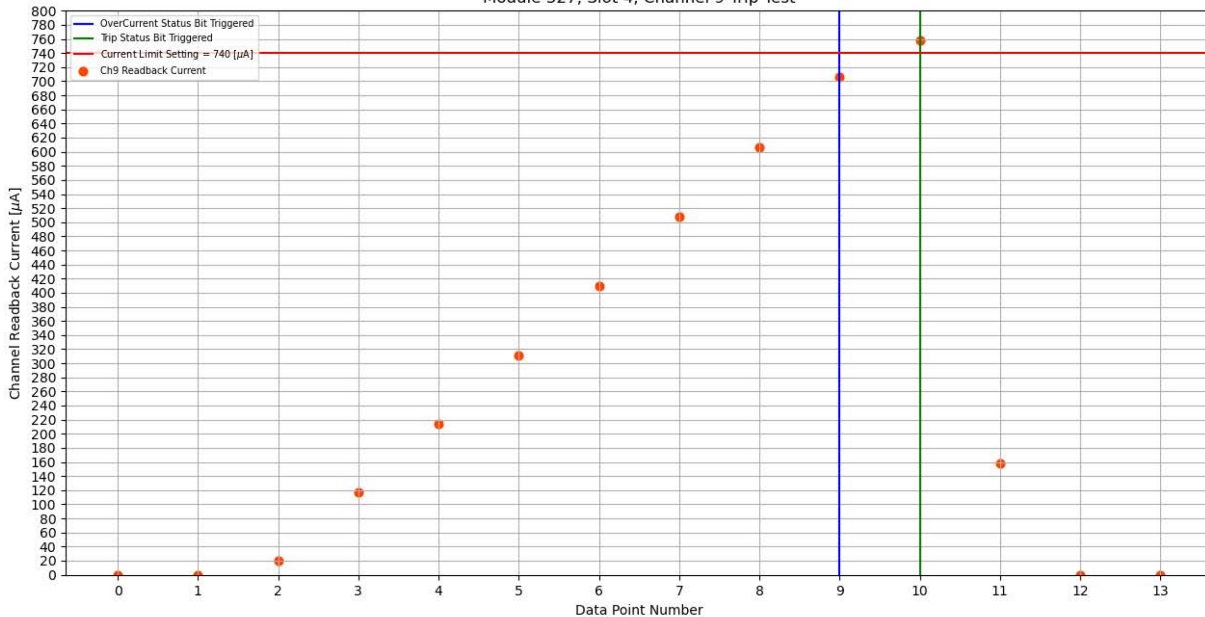
Module 327, Slot 4, Channel 9 Trip Test
