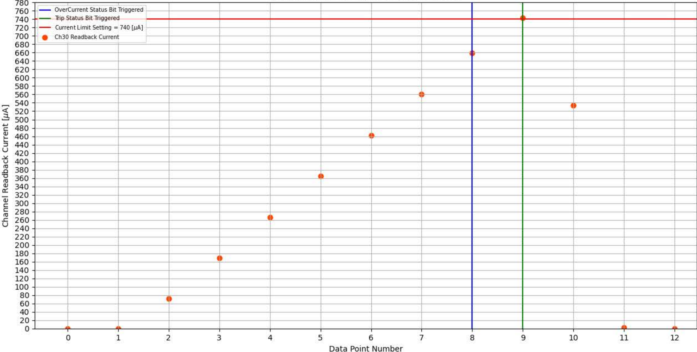
Module 327, Slot 4, Channel 30 Trip Test
