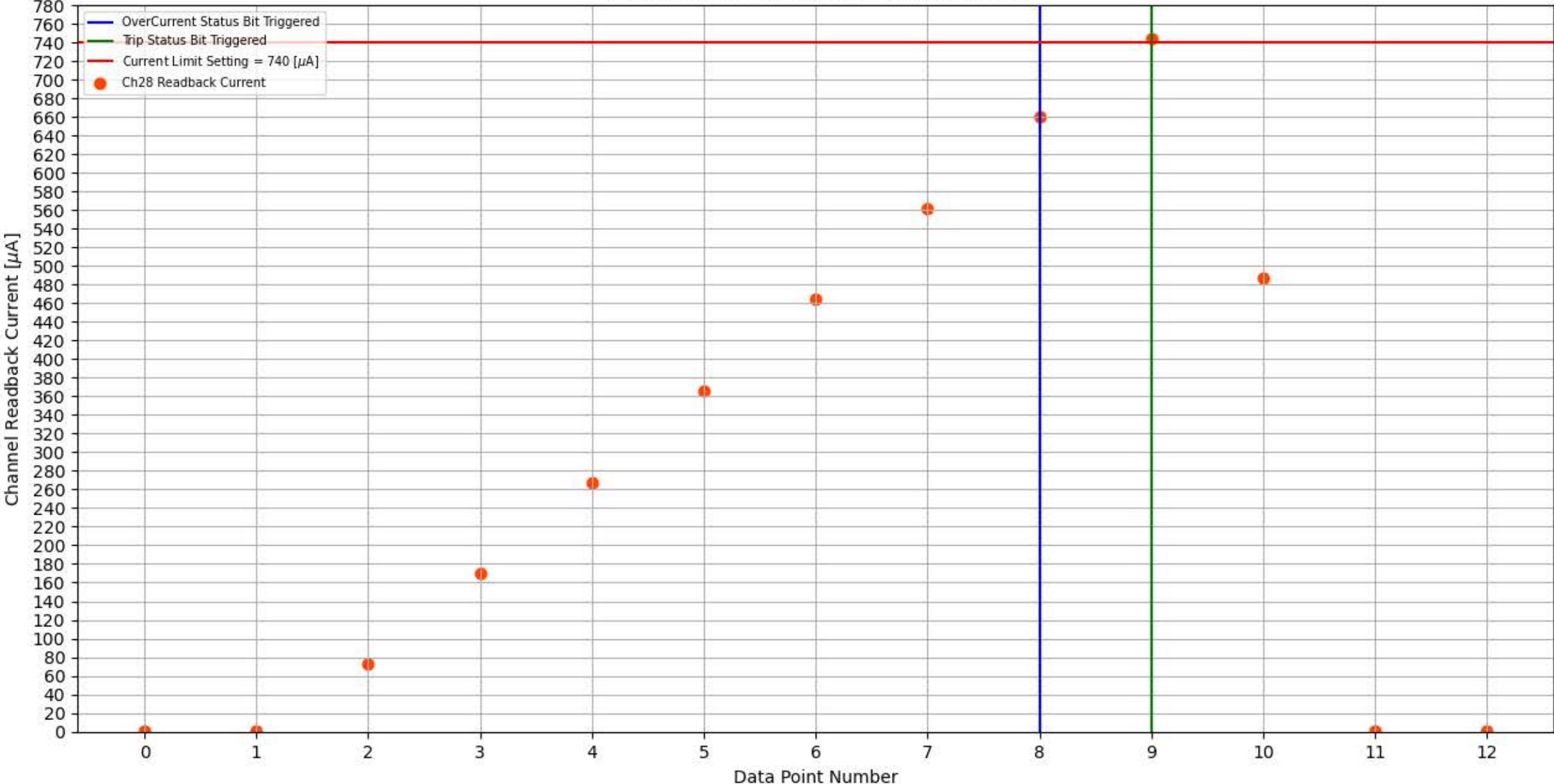
Module 327, Slot 4, Channel 28 Trip Test
