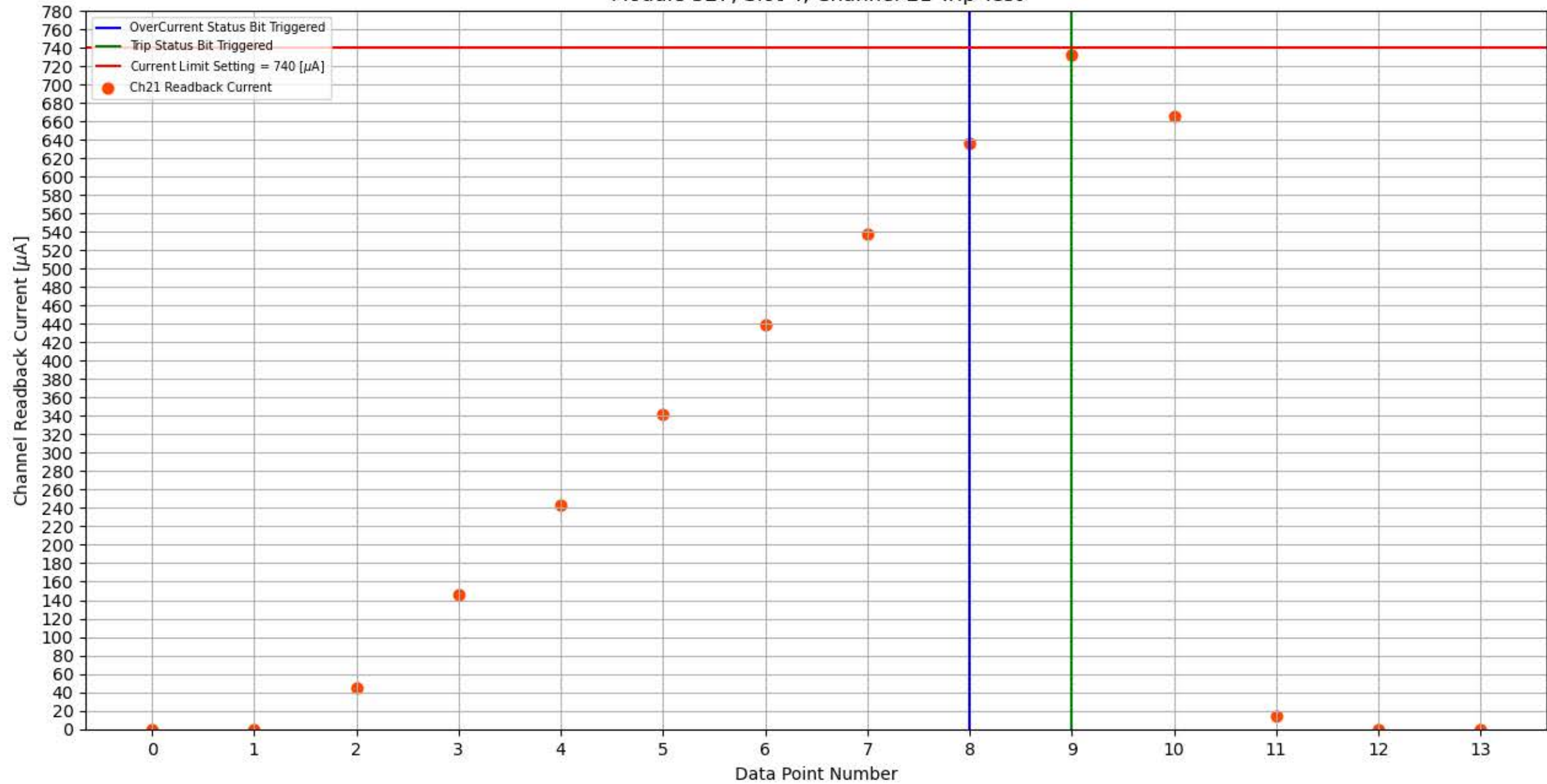
Module 327, Slot 4, Channel 21 Trip Test
