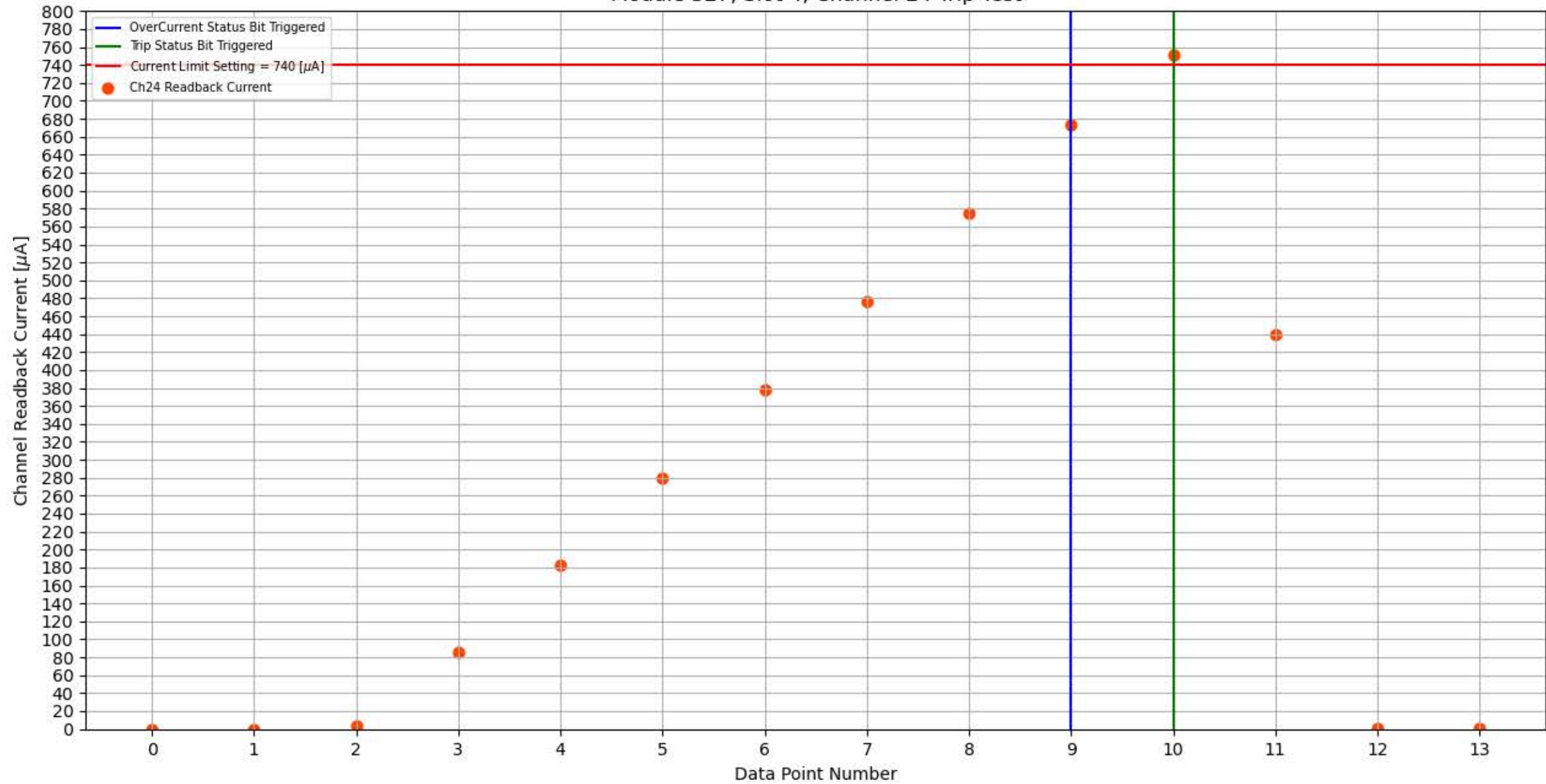
Module 327, Slot 4, Channel 24 Trip Test
