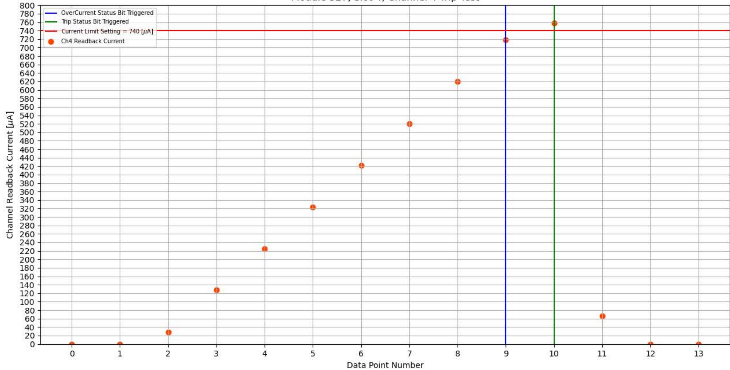
Module 327, Slot 4, Channel 4 Trip Test
