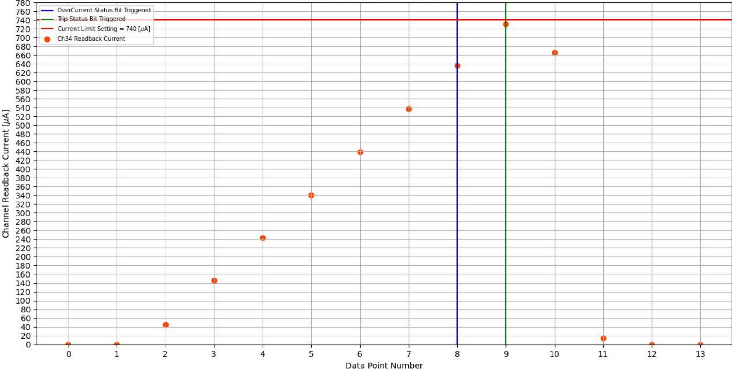
Module 327, Slot 4, Channel 34 Trip Test
