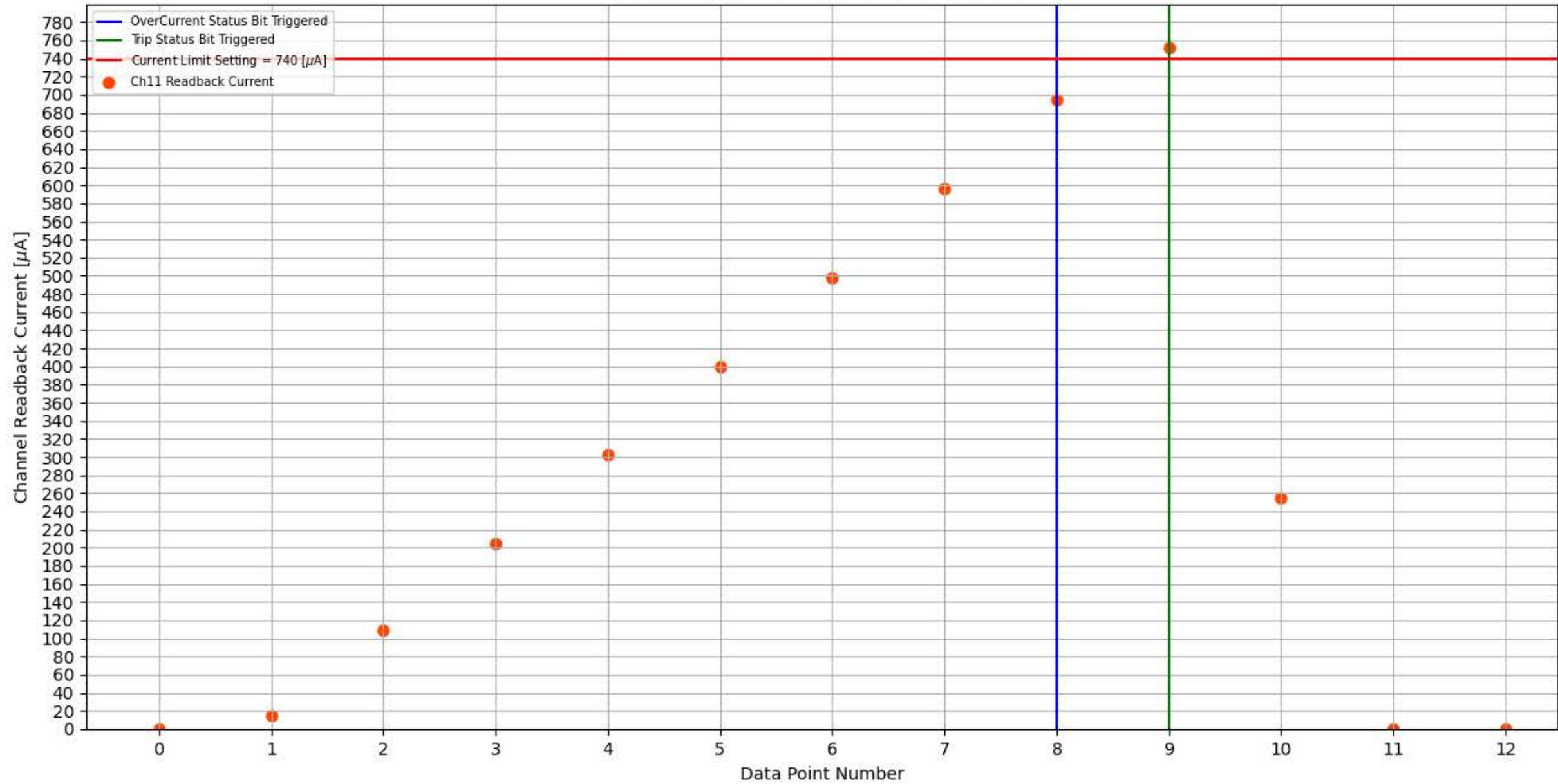
Module 327, Slot 4, Channel 11 Trip Test
