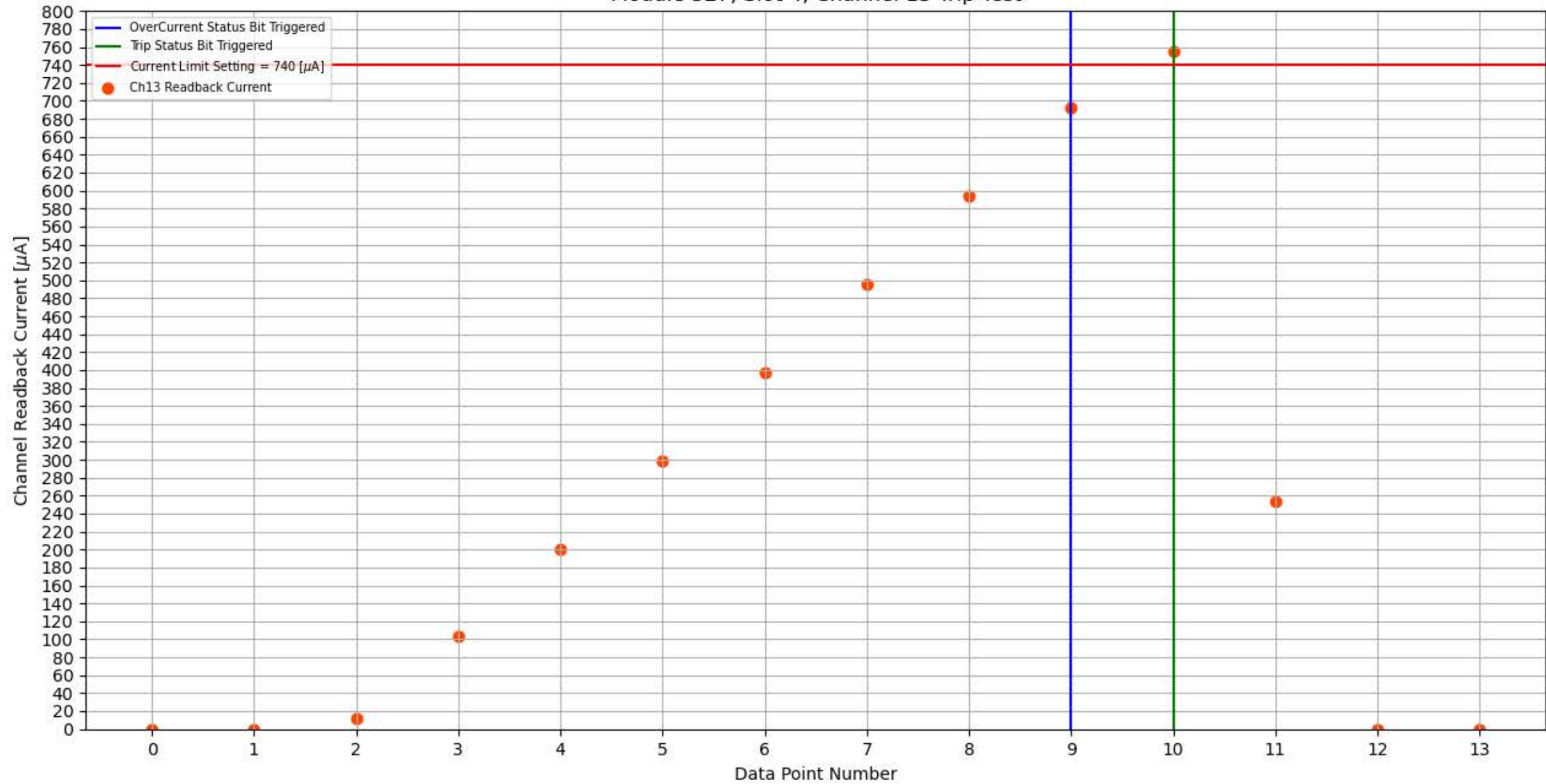
Module 327, Slot 4, Channel 13 Trip Test
