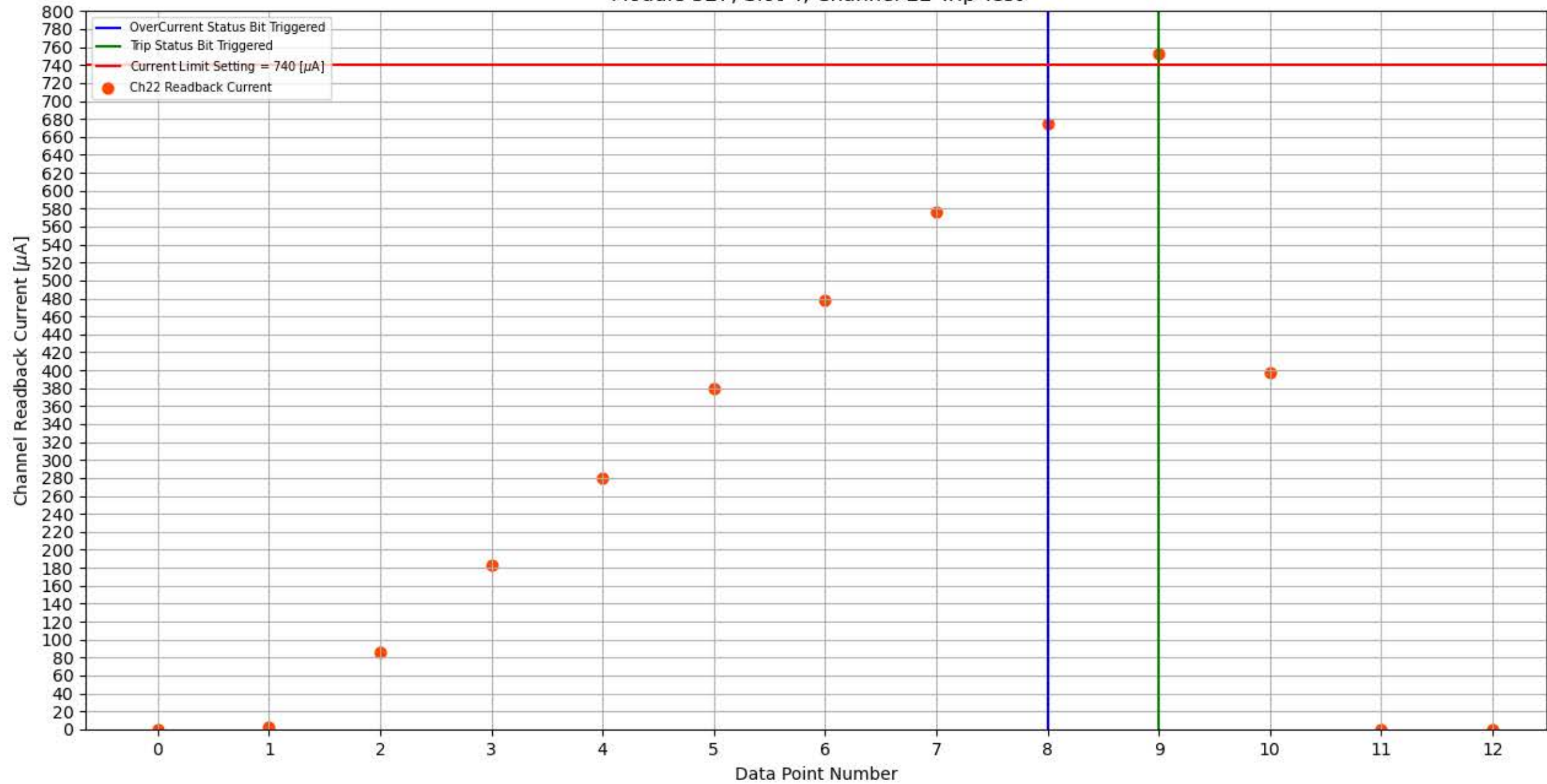
Module 327, Slot 4, Channel 22 Trip Test
