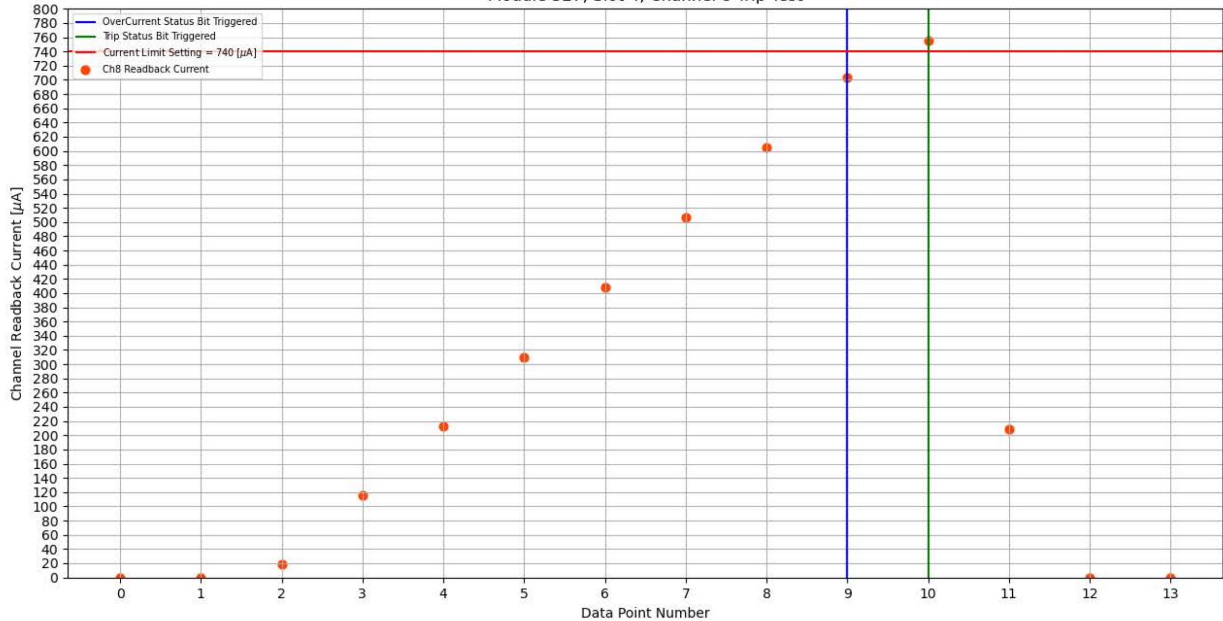
Module 327, Slot 4, Channel 8 Trip Test
