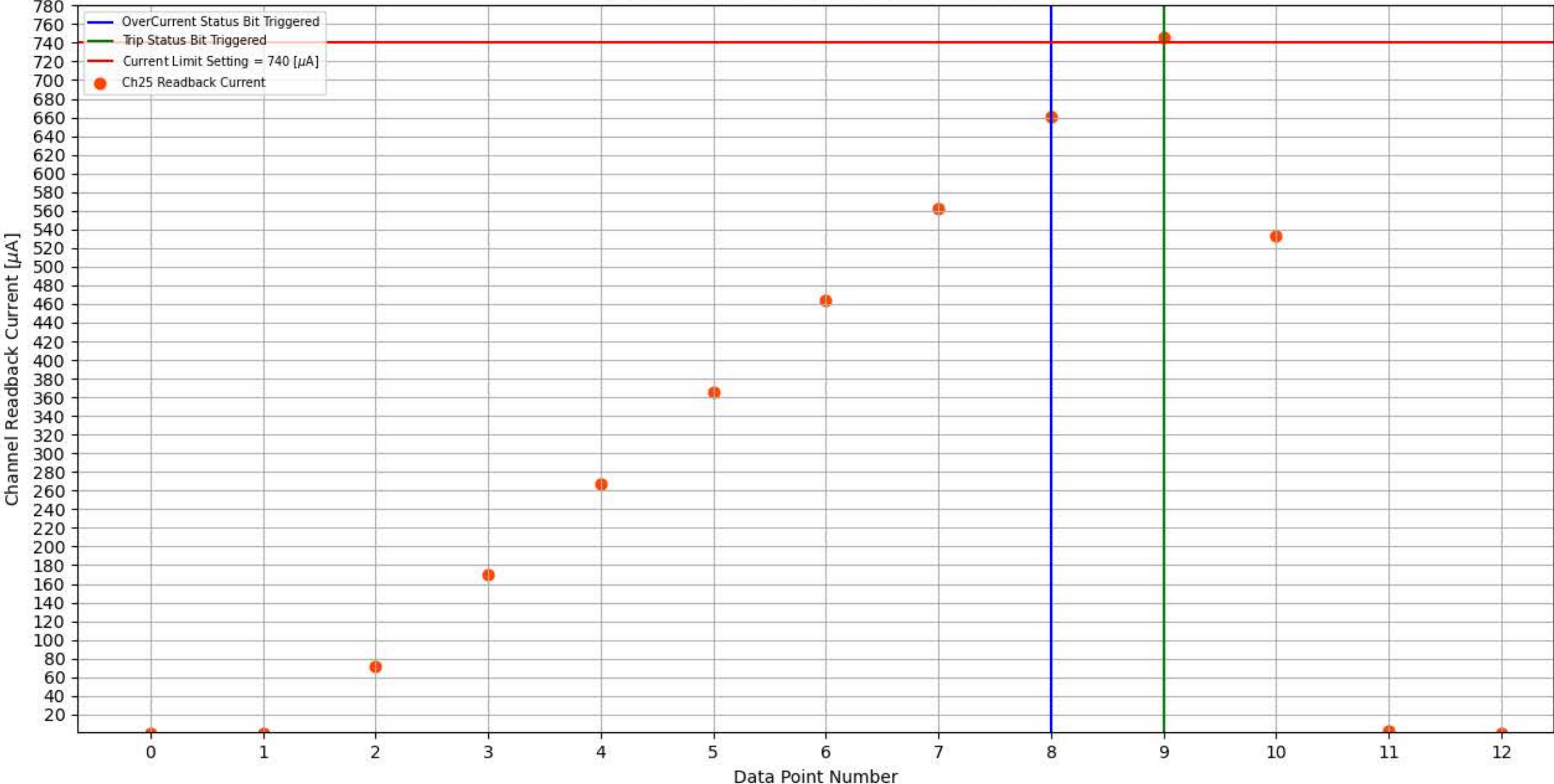
Module 327, Slot 4, Channel 25 Trip Test
