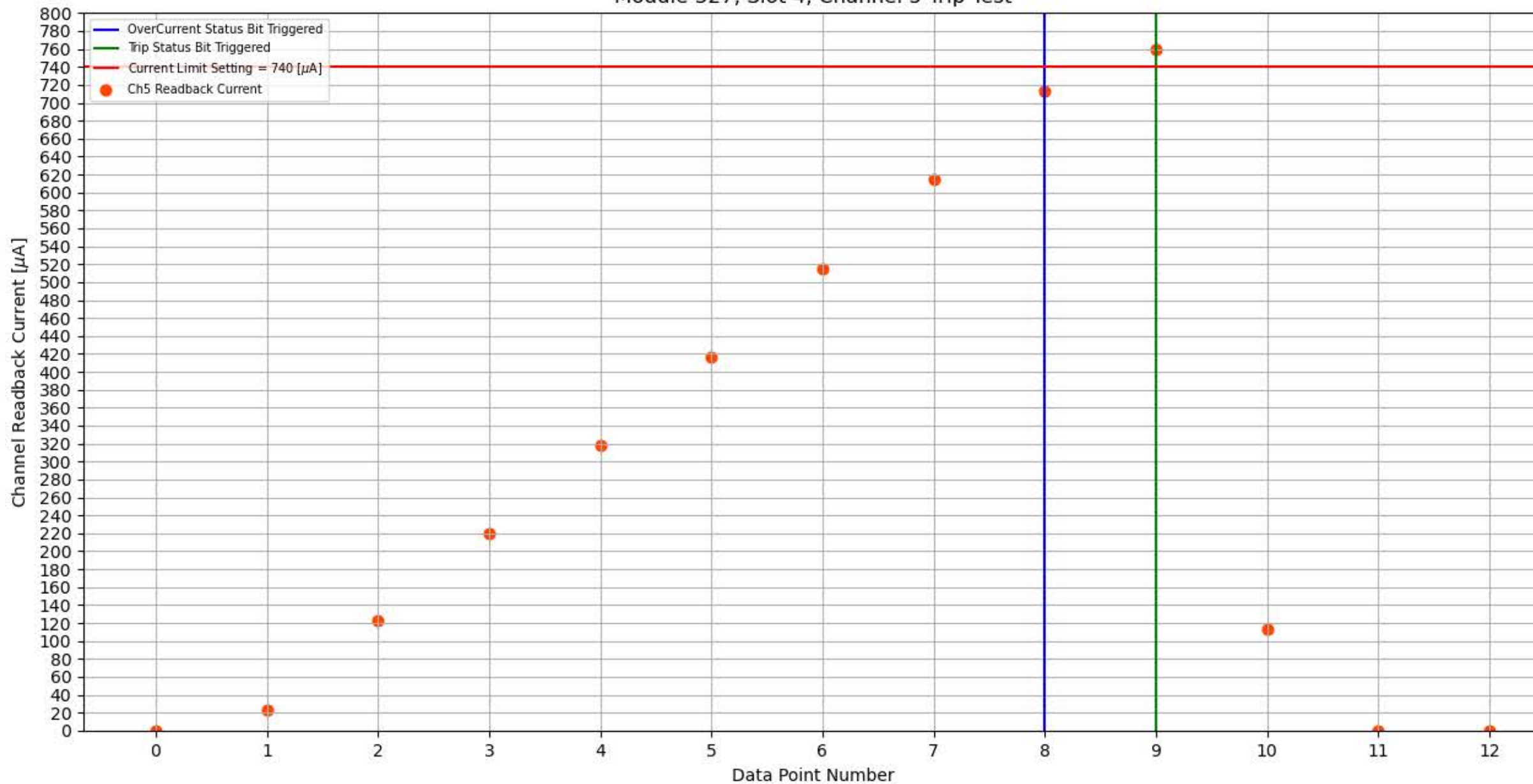
Module 327, Slot 4, Channel 5 Trip Test
