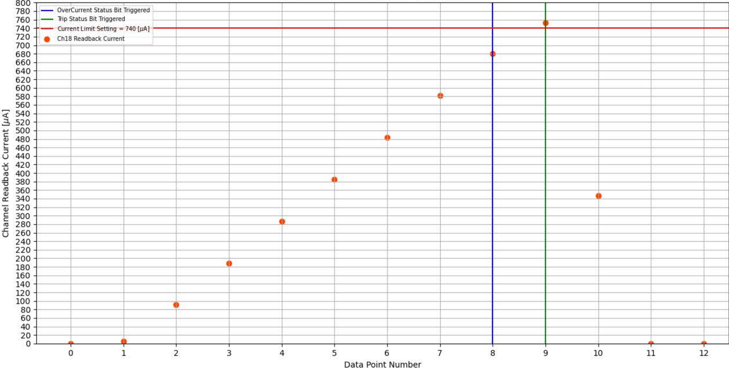
Module 327, Slot 4, Channel 18 Trip Test
