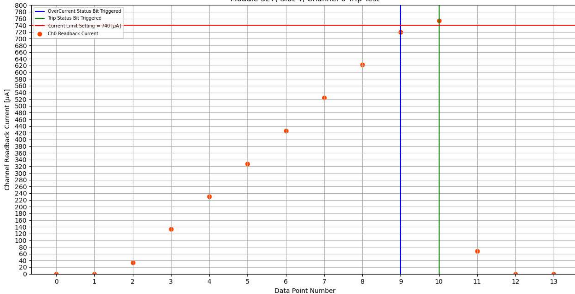
Module 327, Slot 4, Channel 0 Trip Test
