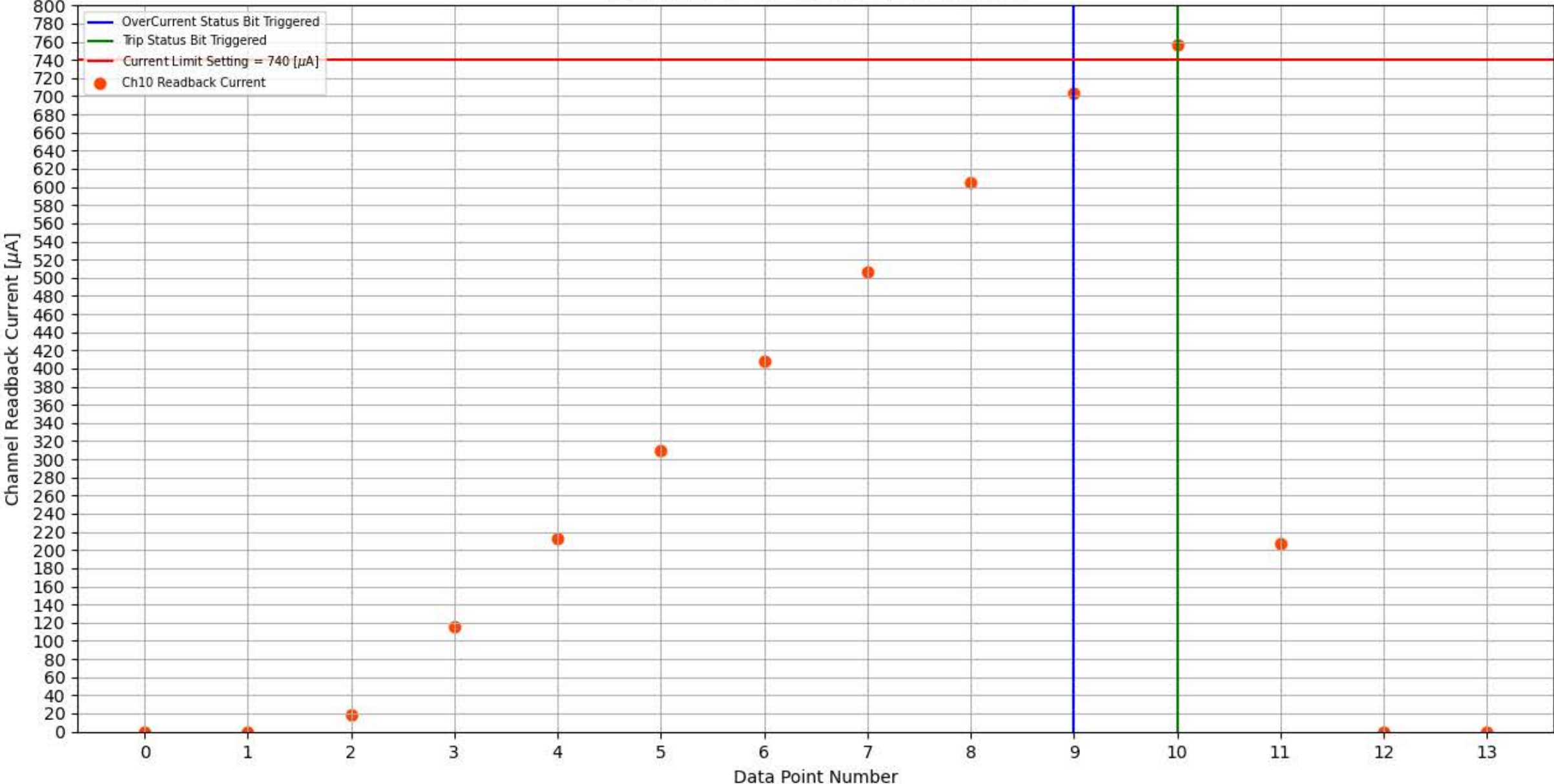
Module 327, Slot 4, Channel 10 Trip Test
