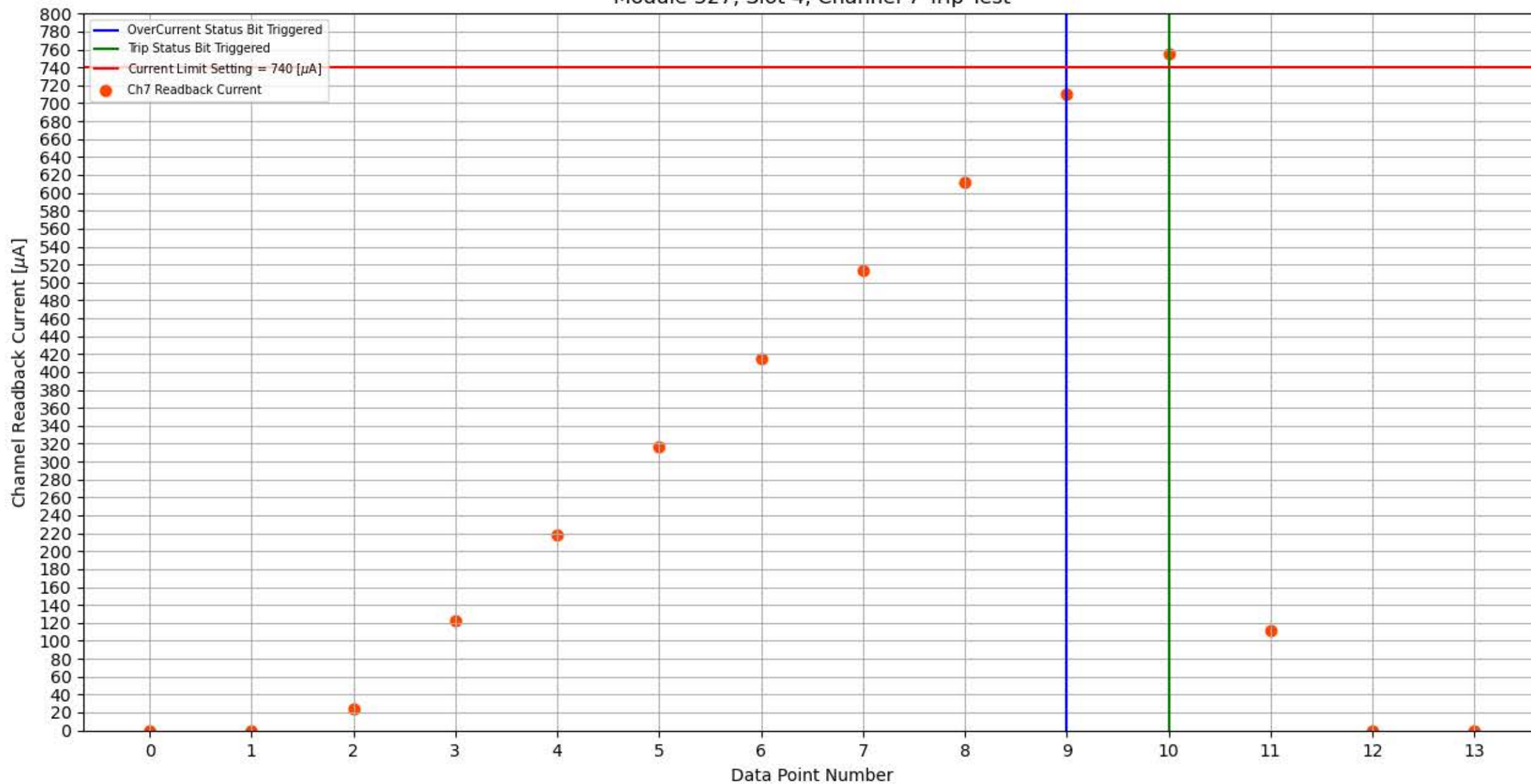
Module 327, Slot 4, Channel 7 Trip Test
