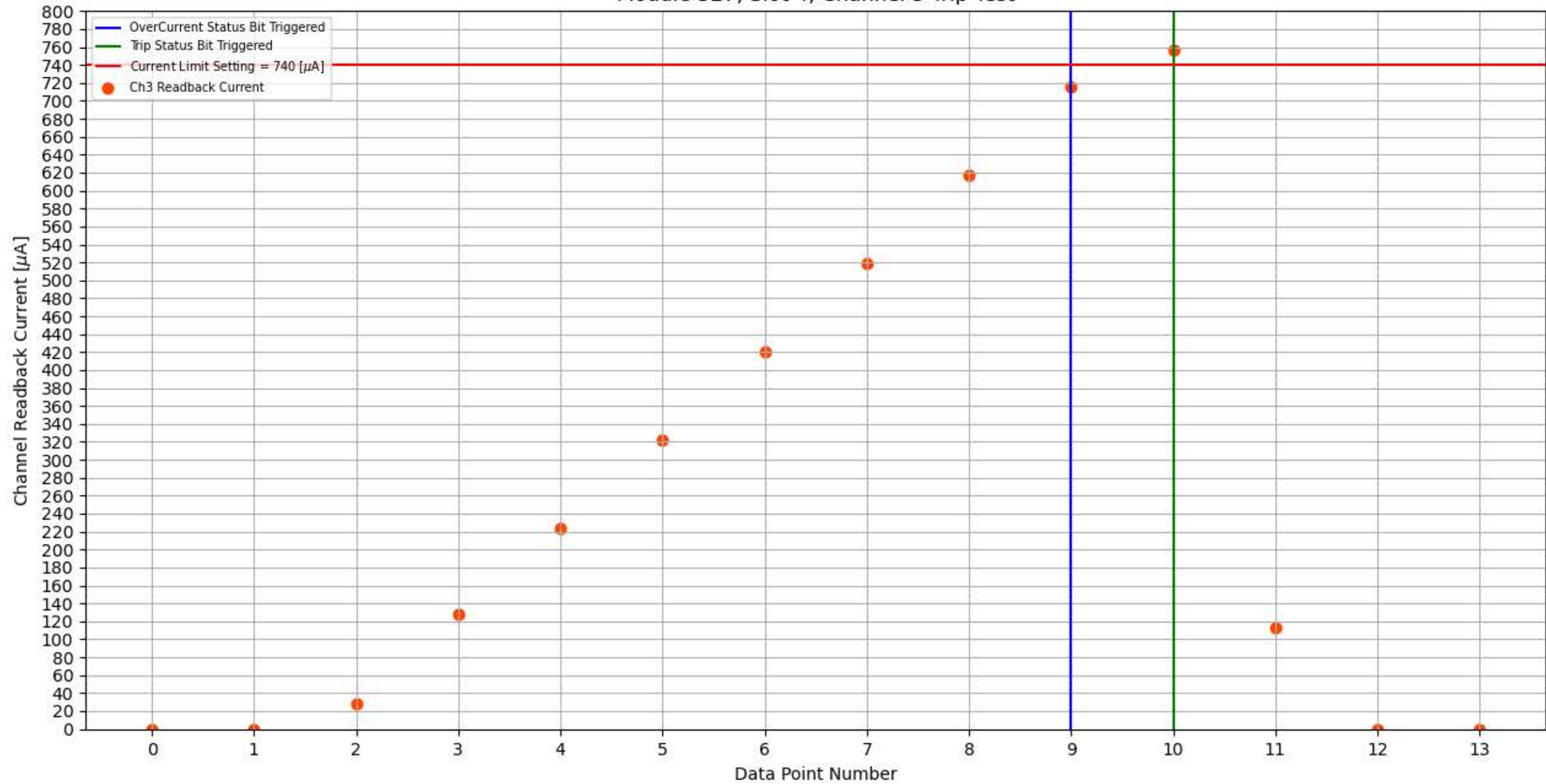
Module 327, Slot 4, Channel 3 Trip Test
