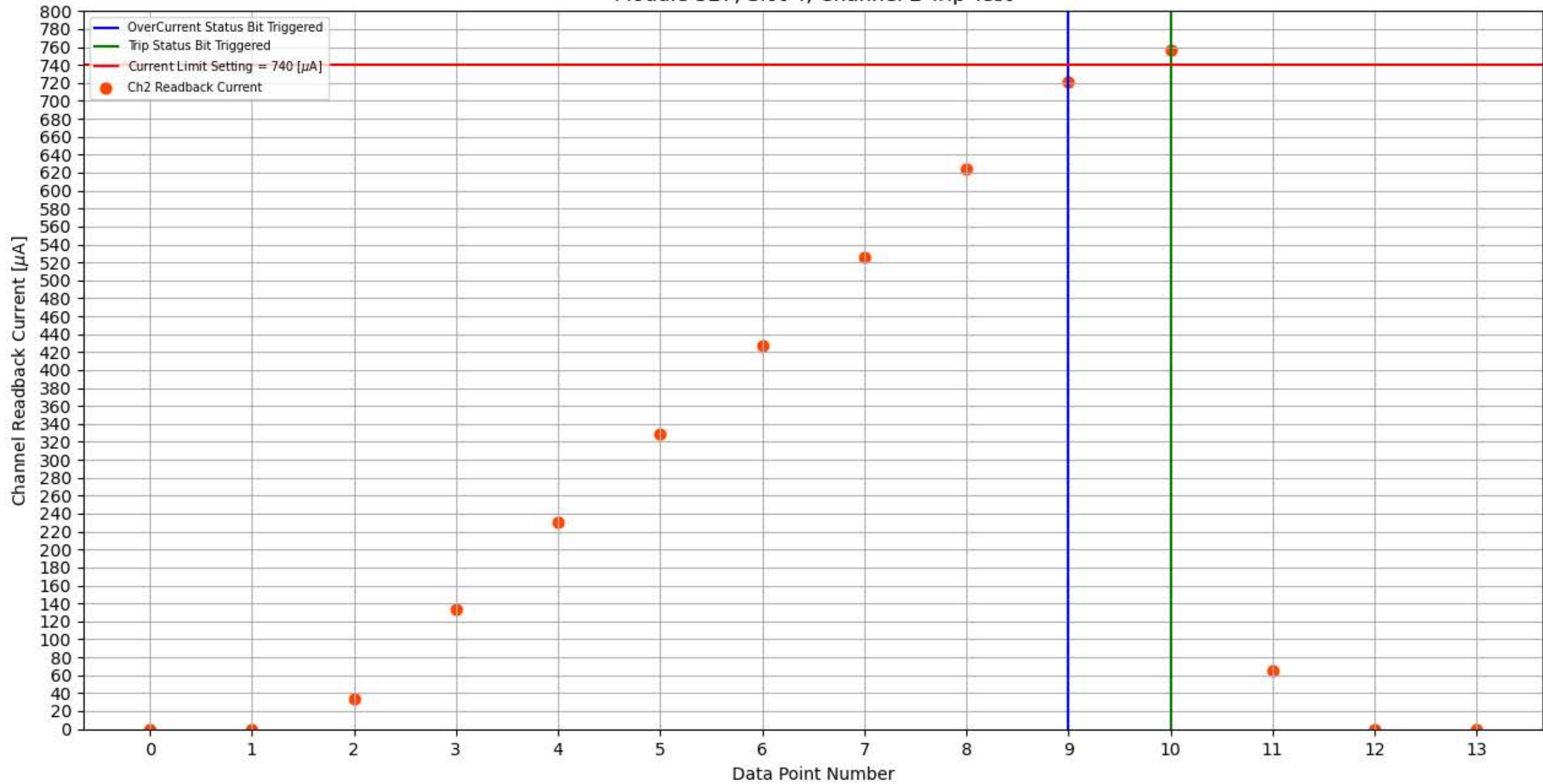
Module 327, Slot 4, Channel 2 Trip Test
