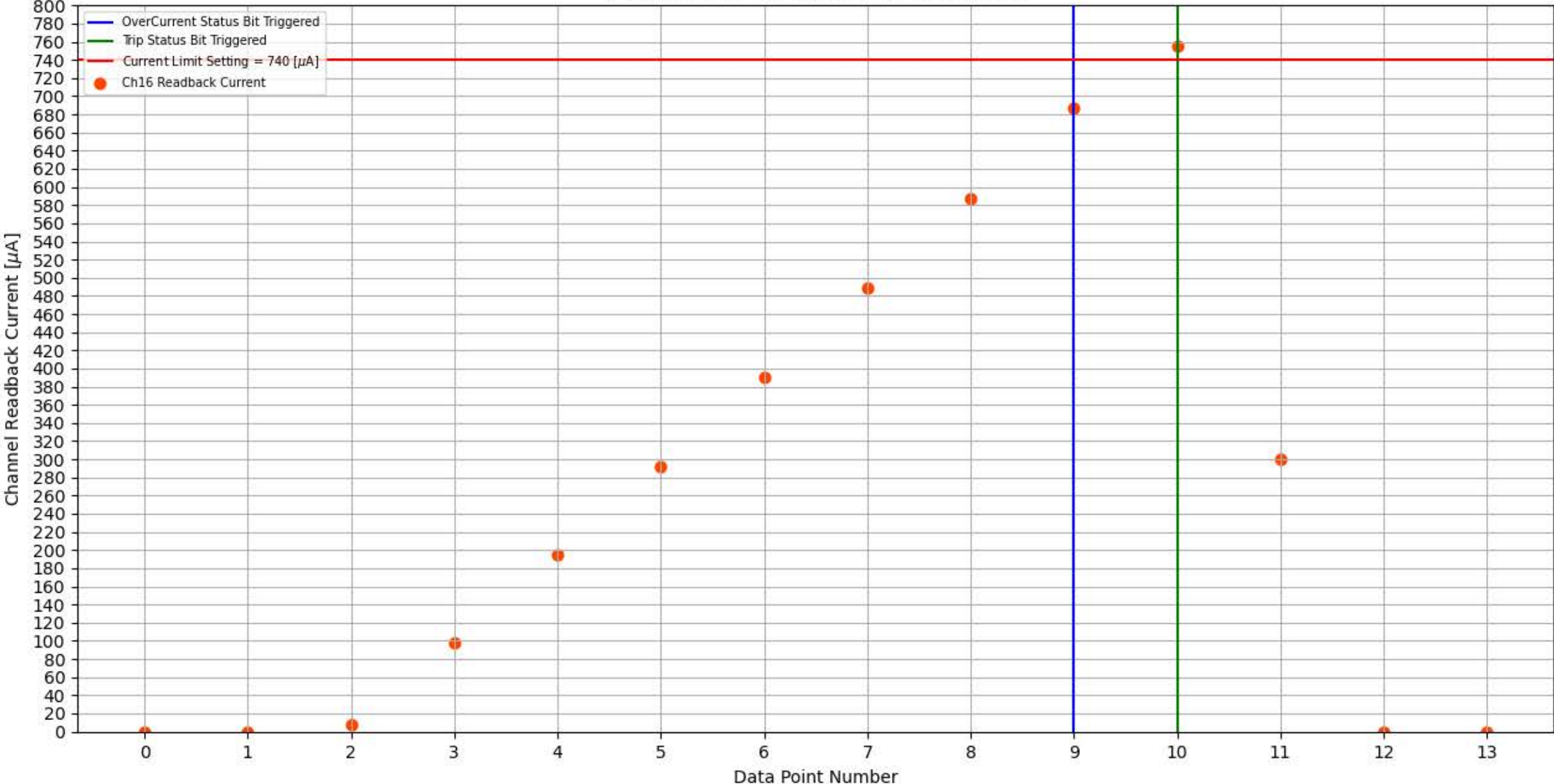
Module 327, Slot 4, Channel 16 Trip Test
