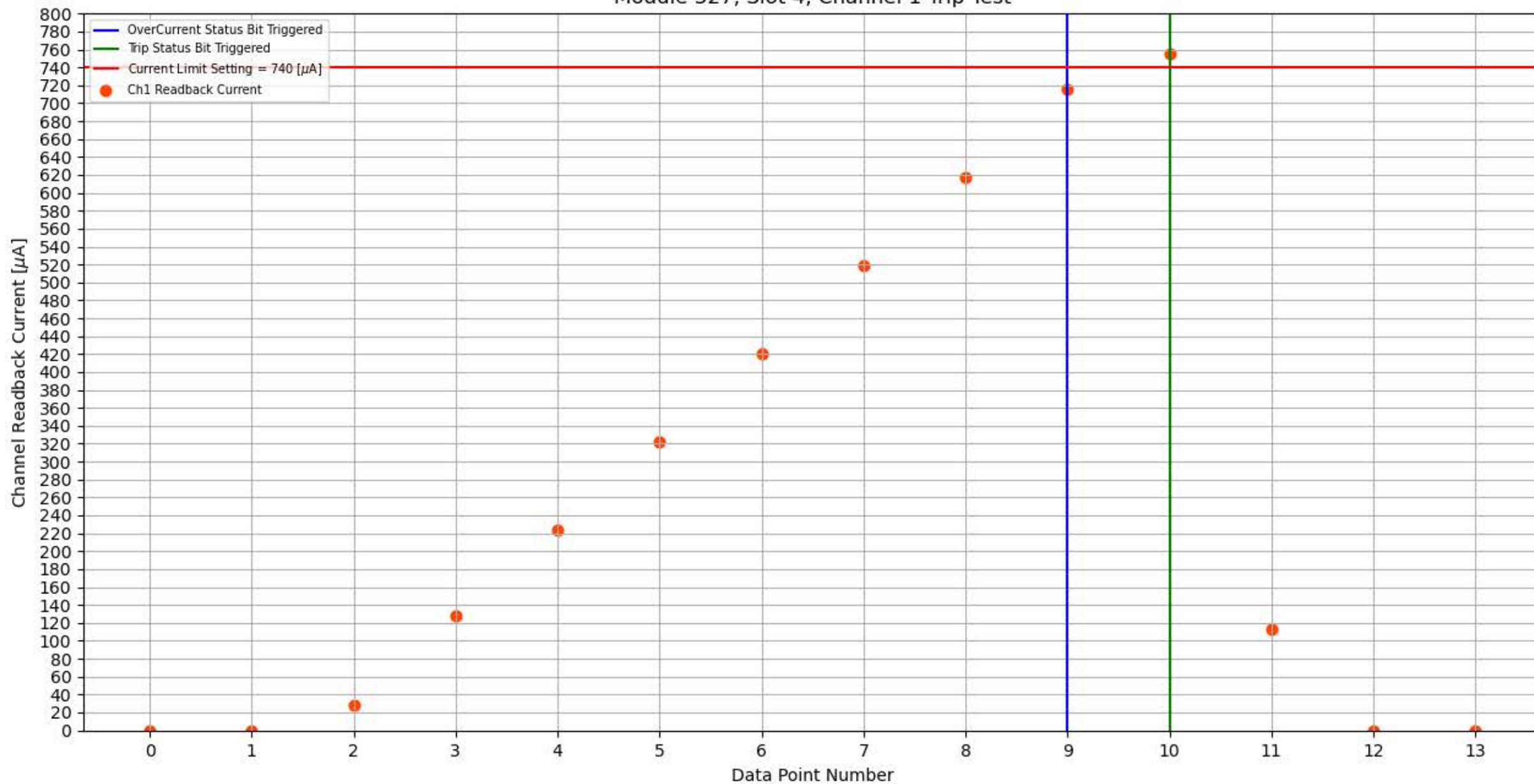
Module 327, Slot 4, Channel 1 Trip Test
