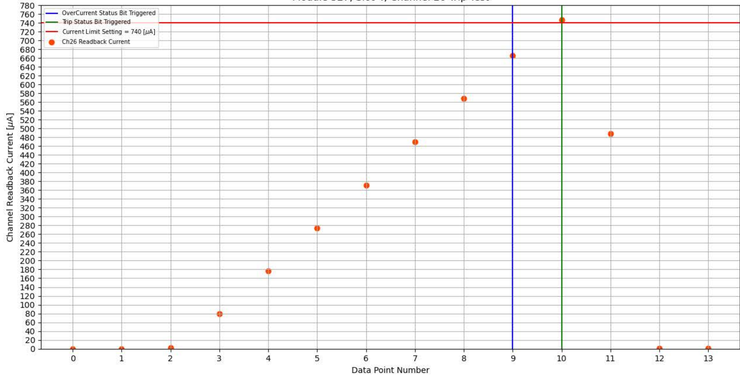
Module 327, Slot 4, Channel 26 Trip Test
