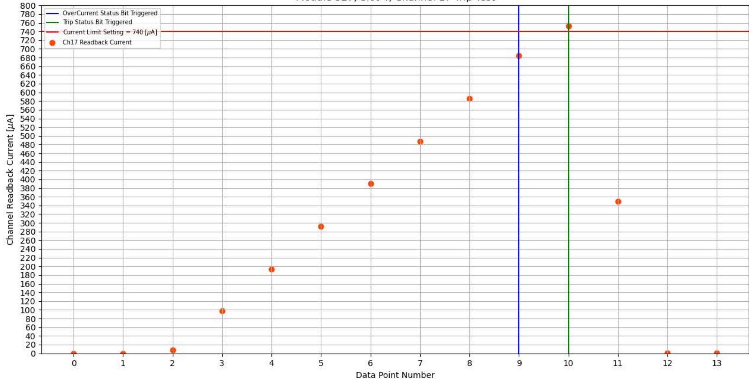
Module 327, Slot 4, Channel 17 Trip Test
