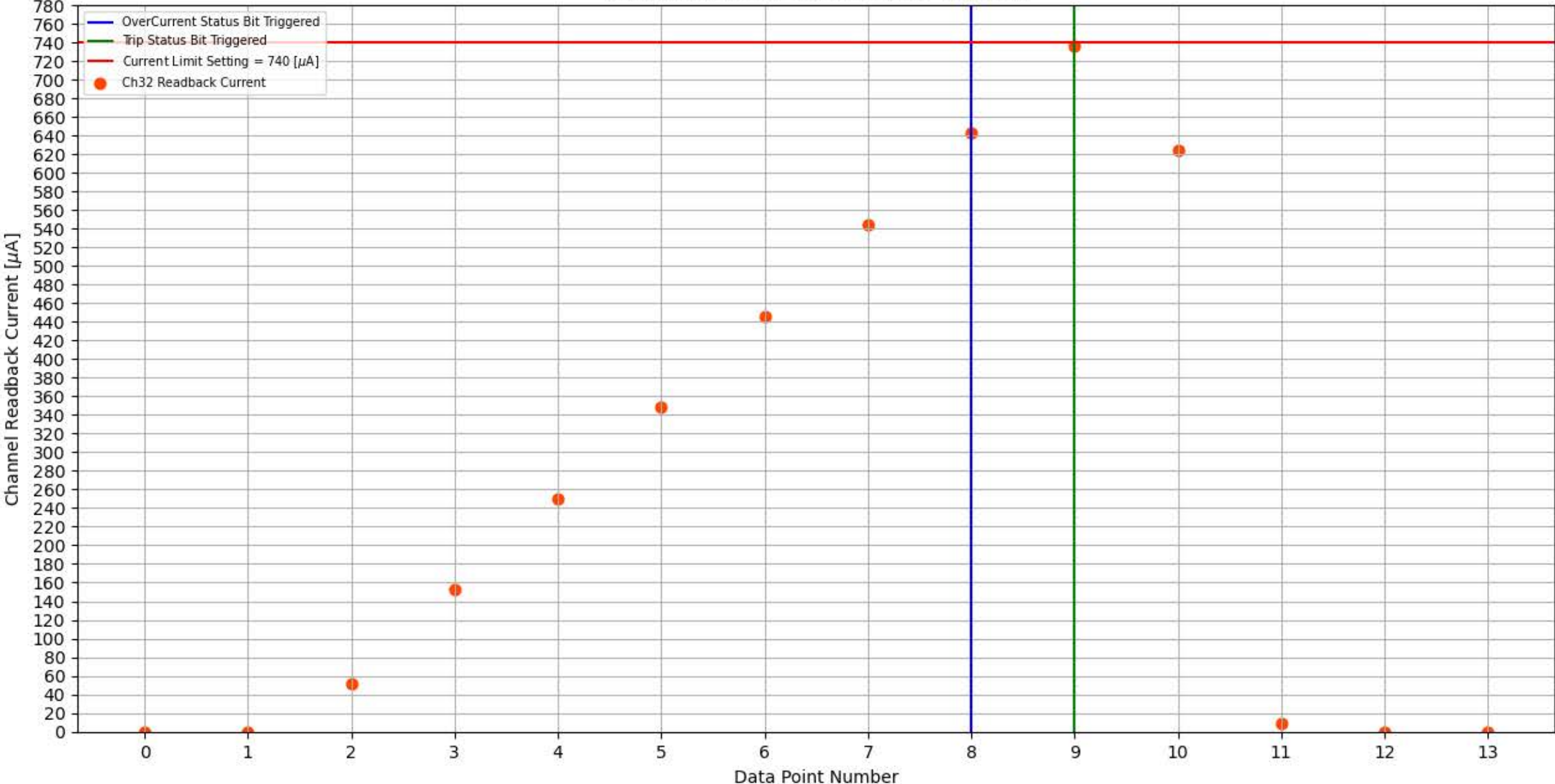
Module 327, Slot 4, Channel 32 Trip Test
