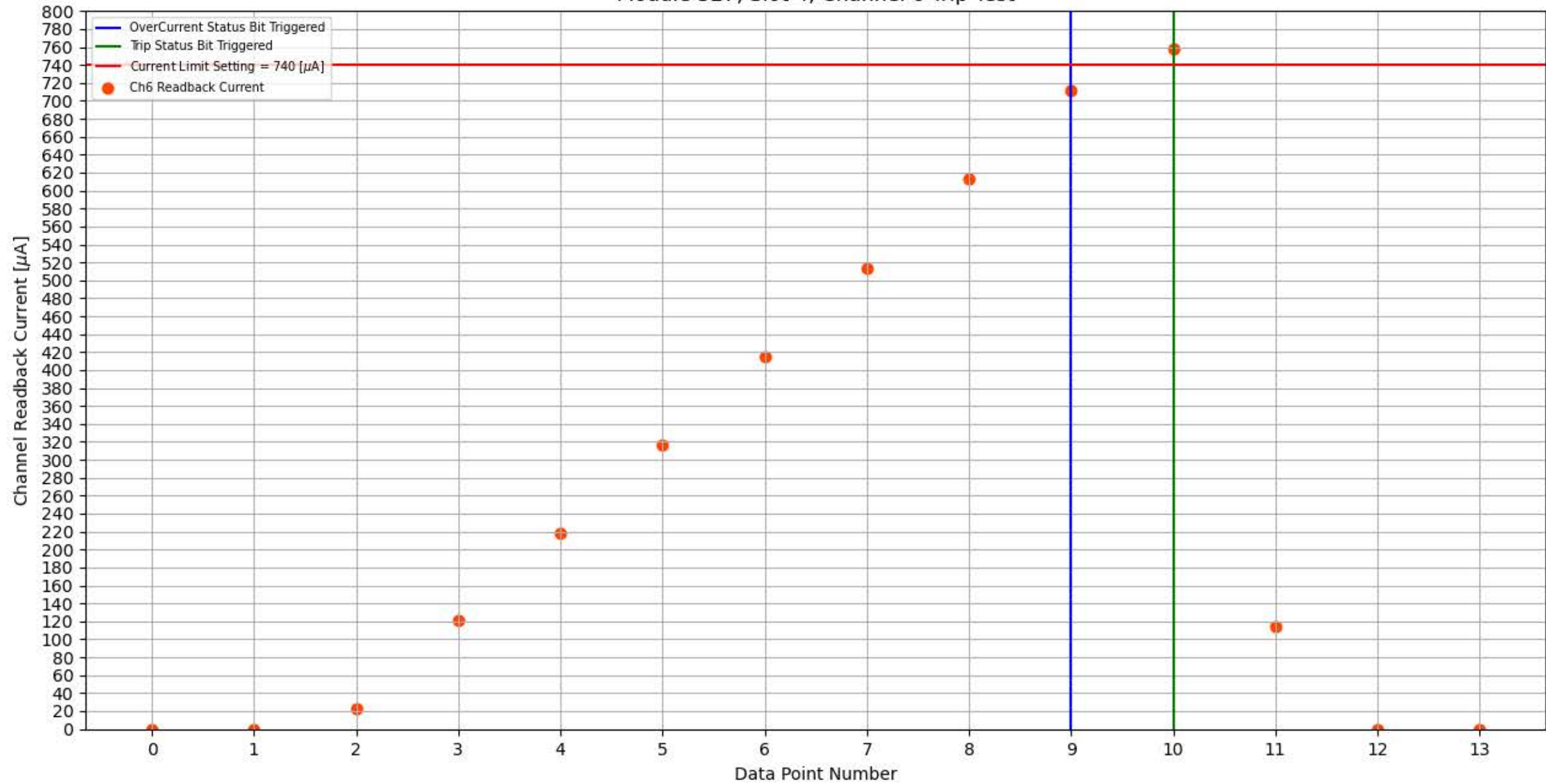
Module 327, Slot 4, Channel 6 Trip Test
