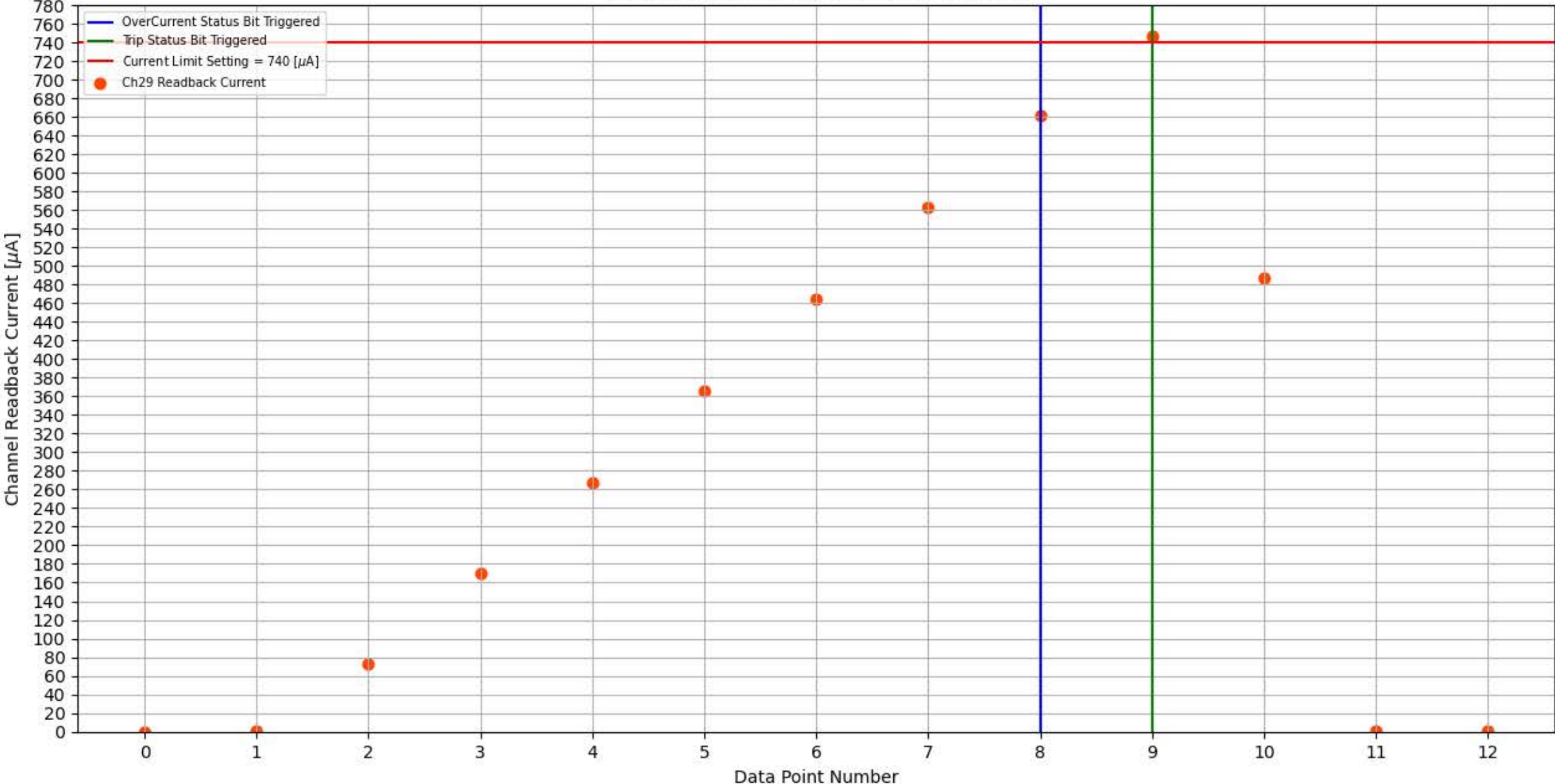
Module 327, Slot 4, Channel 29 Trip Test
